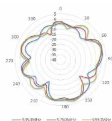
5350-5930 MHz
